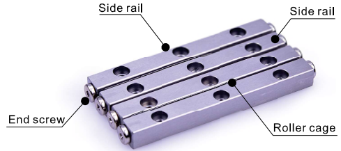
Four-Row Type Of Crossed Roller Way
