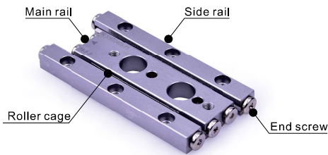
Three-Row Type Of Crossed Roller Way
